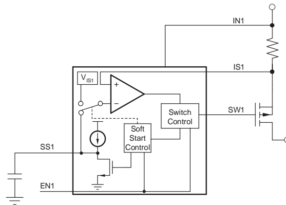
Figure 24. Soft-Start Circuitry
