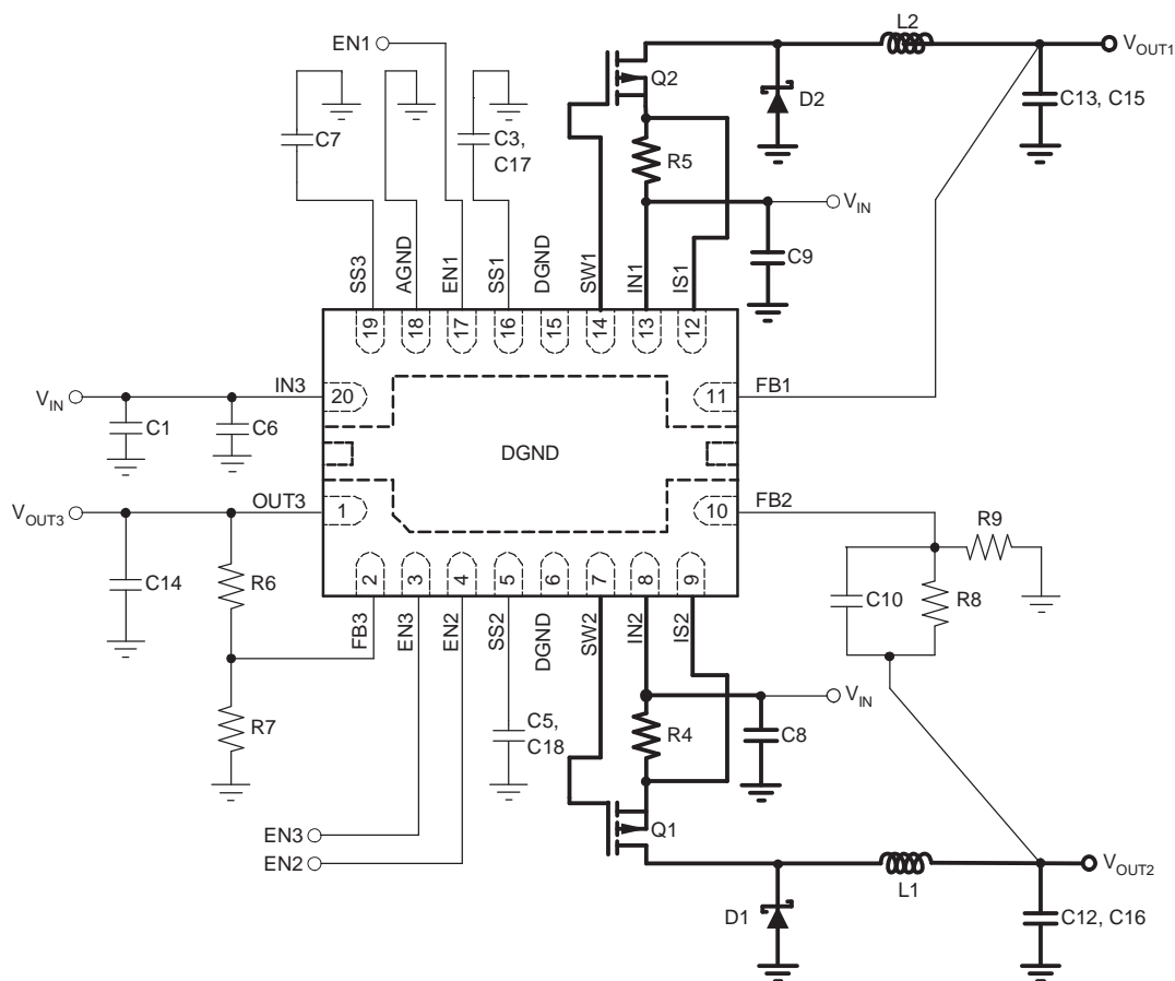
Figure 27. Typical Application Circuit
