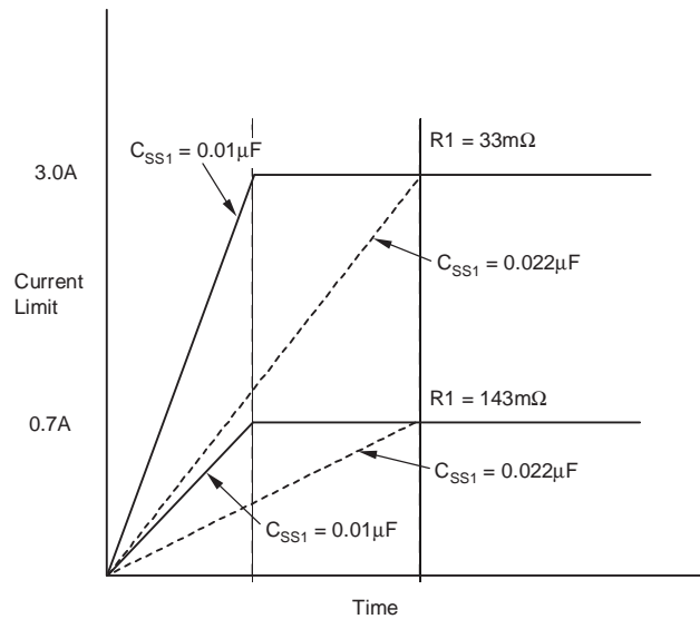
Figure 26. Effects of C_{SS1} and R_1 on Current Ramp Limit
