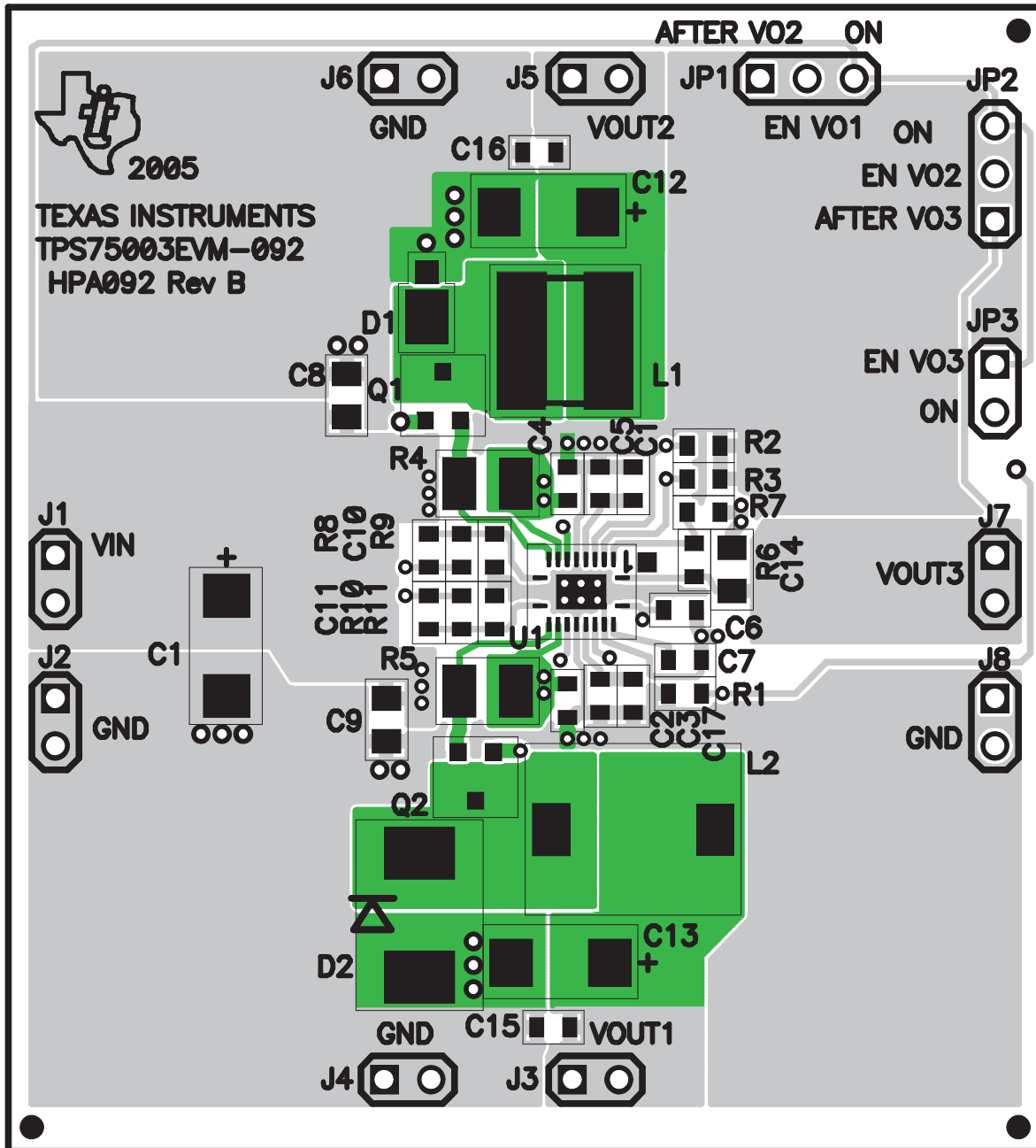
Figure 28. Recommended PCB Layout, Component Side, Top View
