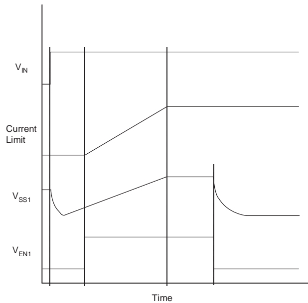
Figure 25. Soft-Start Timing Diagram
