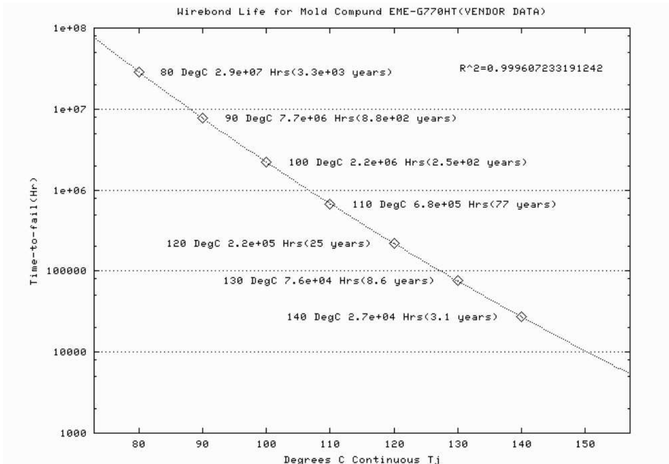
Figure 1. Wirebond Plot
