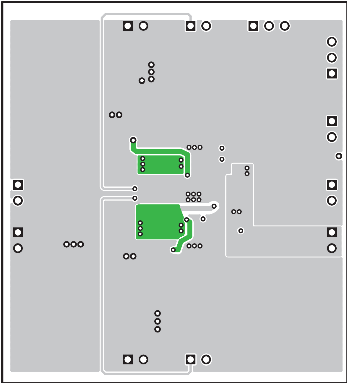
Figure 29. Recommended PCB Layout, Bottom Side, Top View
