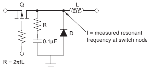
Figure 23. RC Snubber and Series Gate Resistor Used to Minimize Ringing
